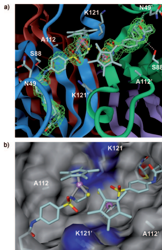
Figure 1. Close-up view of the X-ray crystal structure (PDB: 3pk2) of complex 5 @S112A Sav showing two symmetry-related cofactors in the biotin-binding pocket of the protein tetramer. F_o - F_c omit map colored in green (contoured at 3 \sigma ) and anomalous difference density map (5 \sigma ) in red (a). Surface representation with basic residues in blue, acidic in red, polar and apolar in gray (b); (chloride: yellow sphere).
